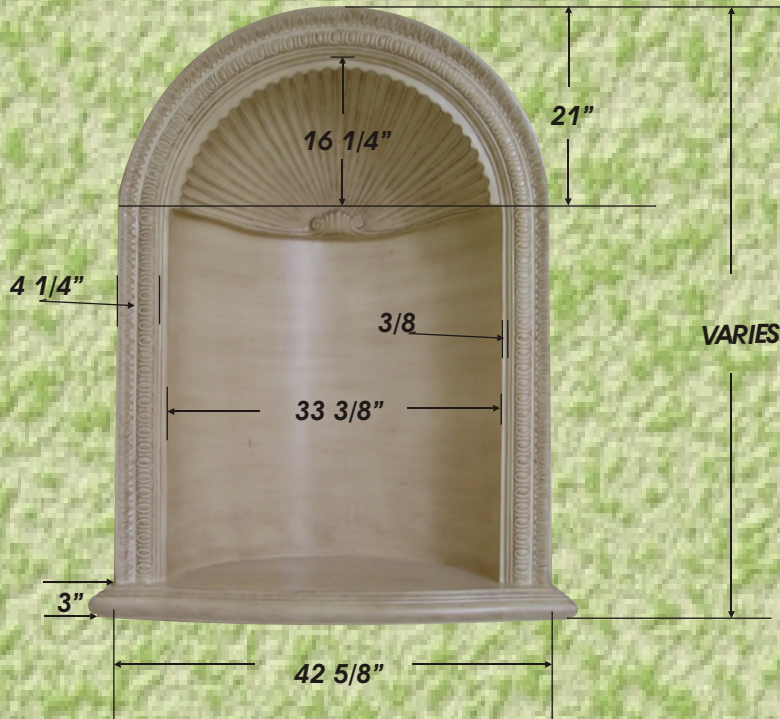
NICHE #100 DEPTH 16 1/4"
